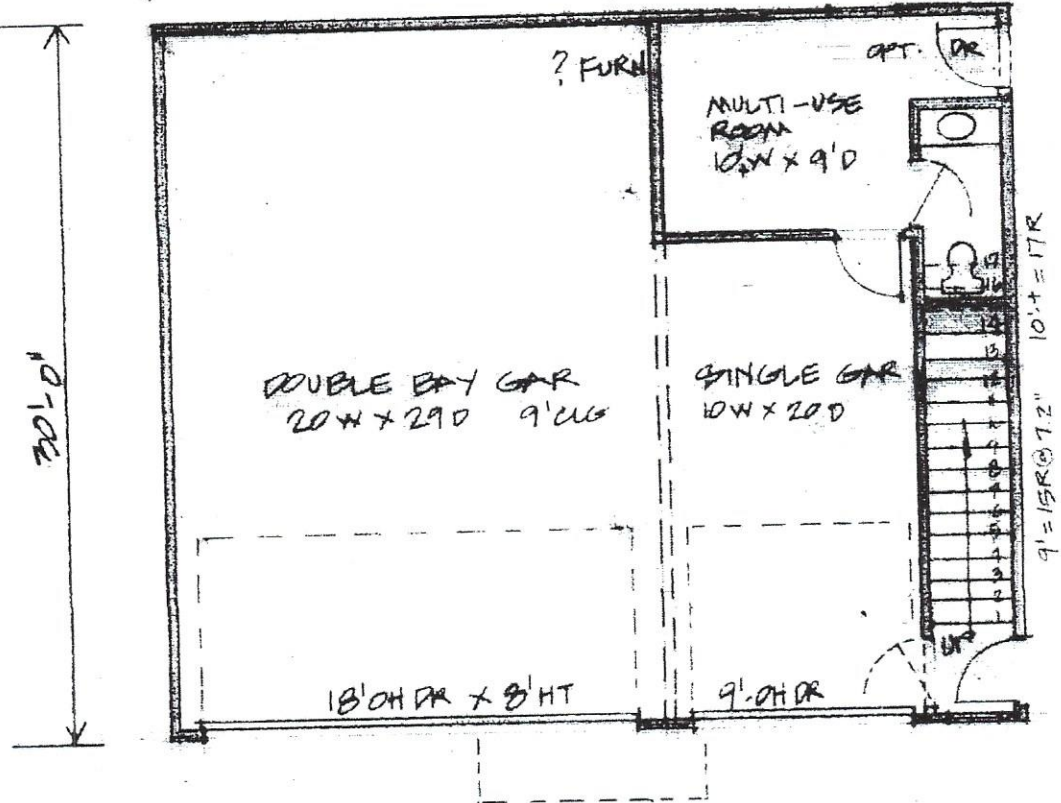
MAIN-FIRST FLOOR PLAN 1/8" = 1'-0"
