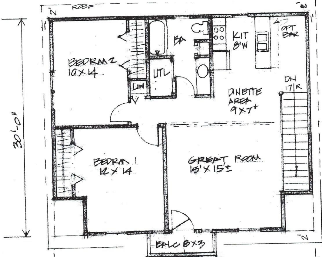
SECOND FLOOR PLAN 1/8" = 1'-0" 35' (OR 34') ±
