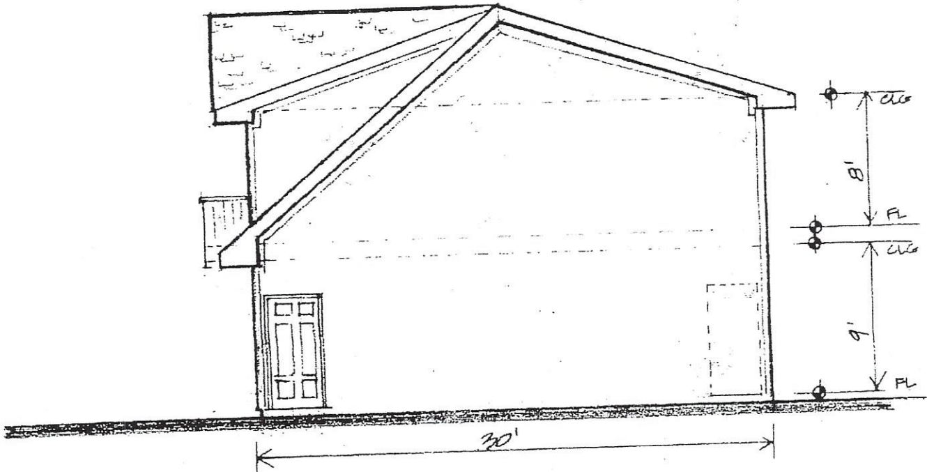
WEST-SIDE ELEVATION \frac{1}{8}'' = 1'-0''
